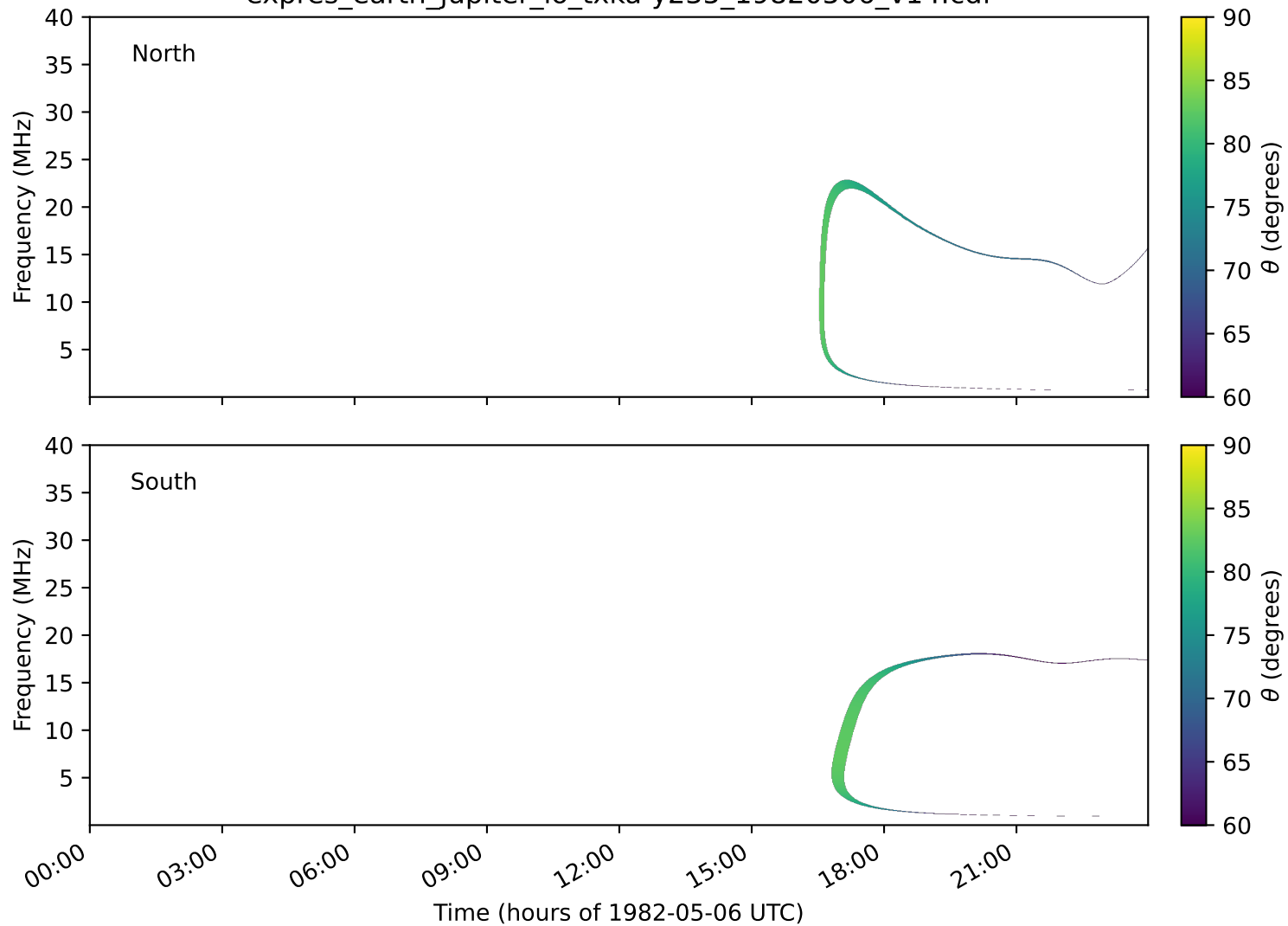
expres_earth_jupiter_io_txka-y235_19820506_v14.cdf
