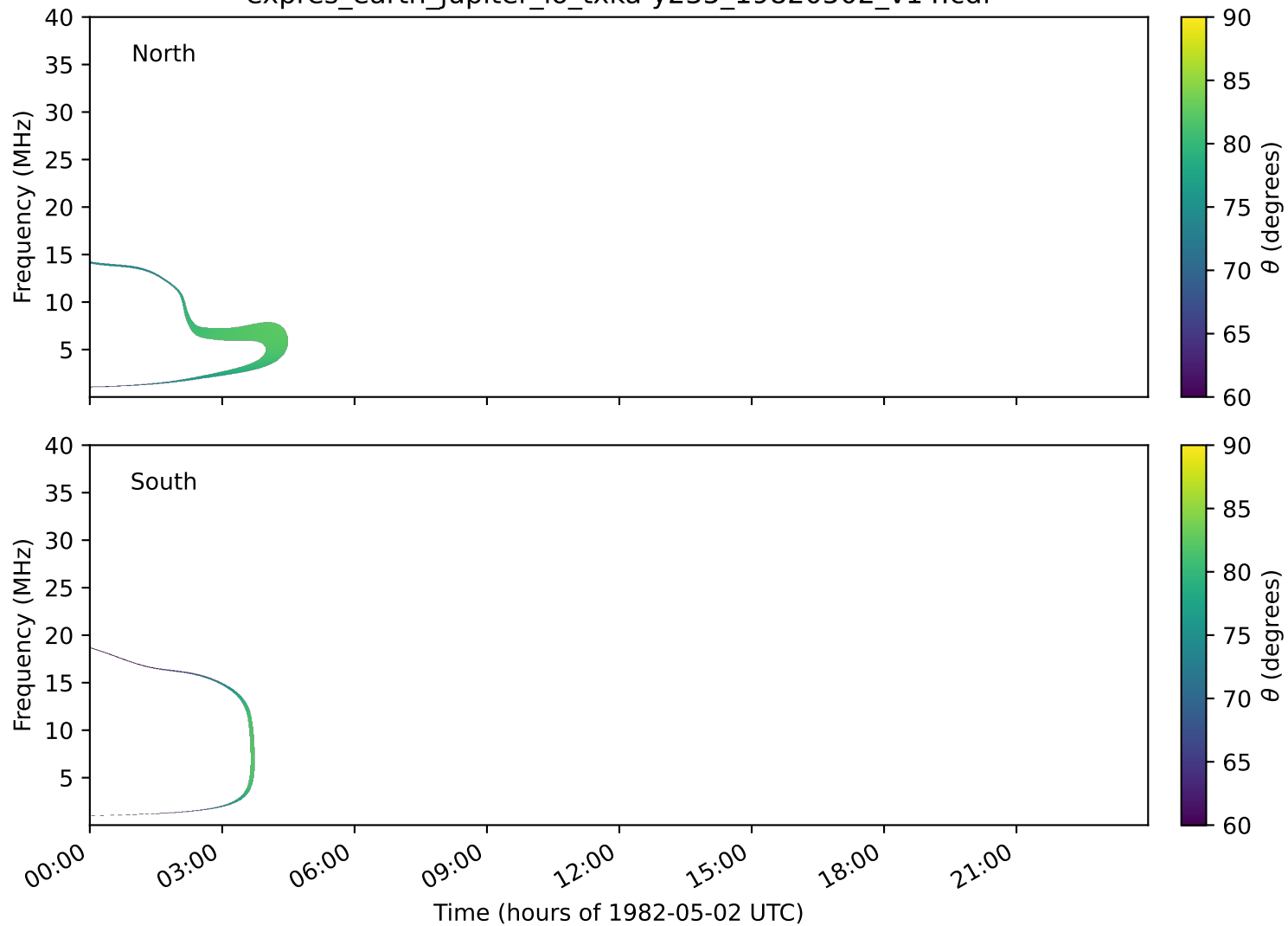
expres_earth_jupiter_io_txka-y235_19820502_v14.cdf
