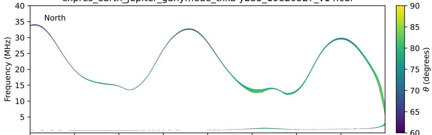
expres_earth_jupiter_ganymede_txka-y235_19820527_v14.cdf
