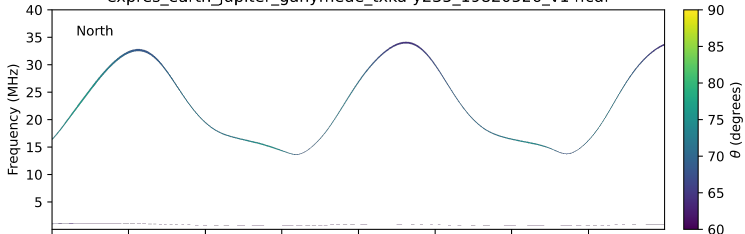
expres_earth_jupiter_ganymede_txka-y235_19820526_v14.cdf
