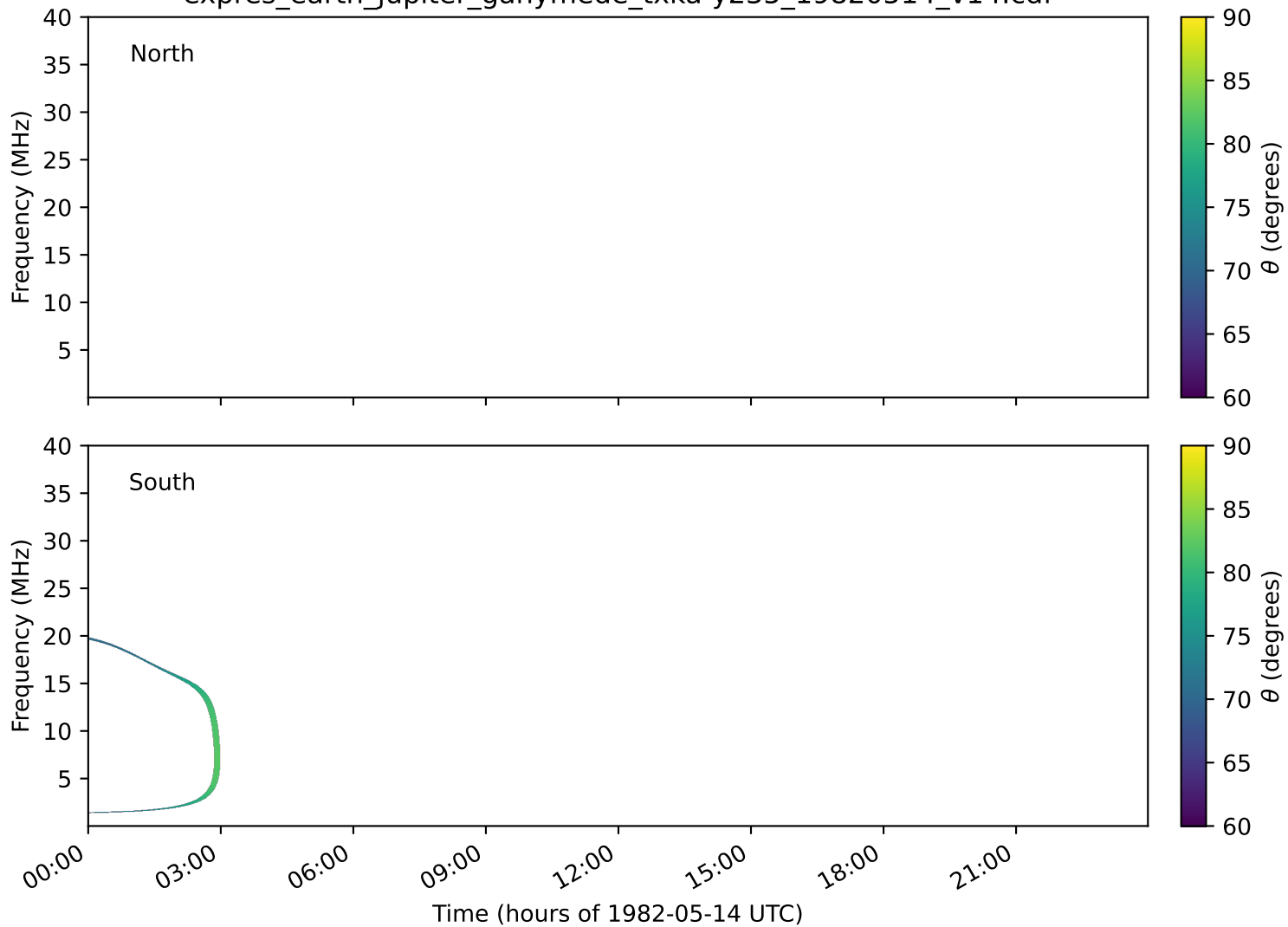
expres_earth_jupiter_ganymede_txka-y235_19820514_v14.cdf
