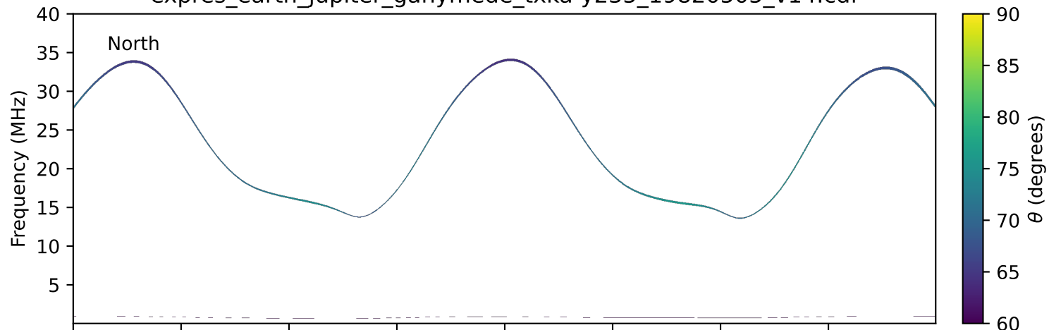
expres_earth_jupiter_ganymede_txka-y235_19820505_v14.cdf
