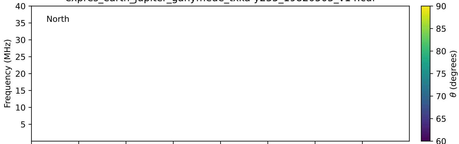
expres_earth_jupiter_ganymede_txka-y235_19820503_v14.cdf
