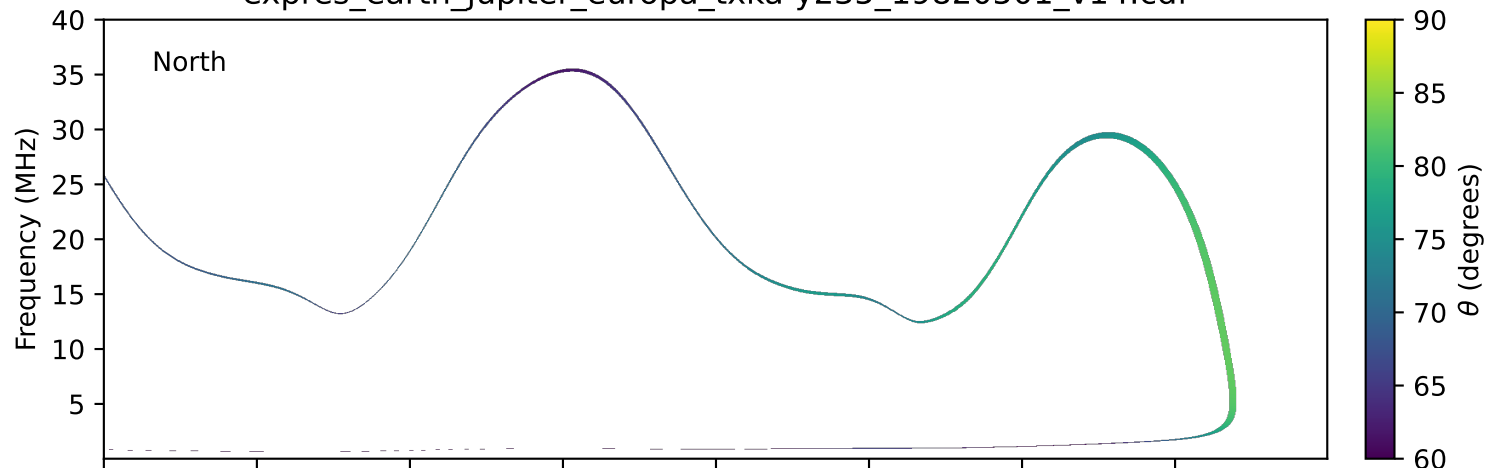
expres_earth_jupiter_europa_txka-y235_19820501_v14.cdf
