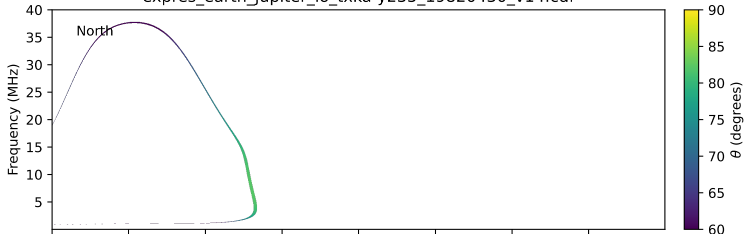
expres_earth_jupiter_io_txka-y235_19820430_v14.cdf
