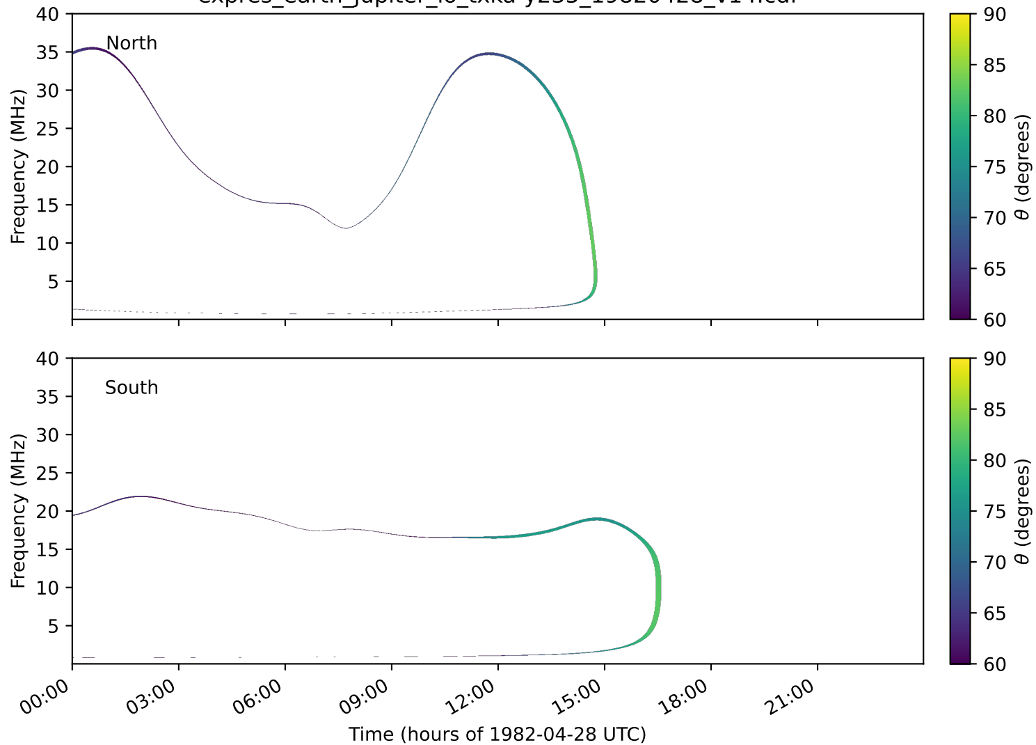
expres_earth_jupiter_io_txka-y235_19820428_v14.cdf
