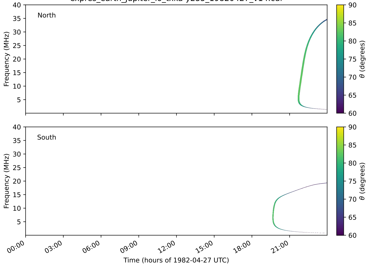
expres_earth_jupiter_io_txka-y235_19820427_v14.cdf
