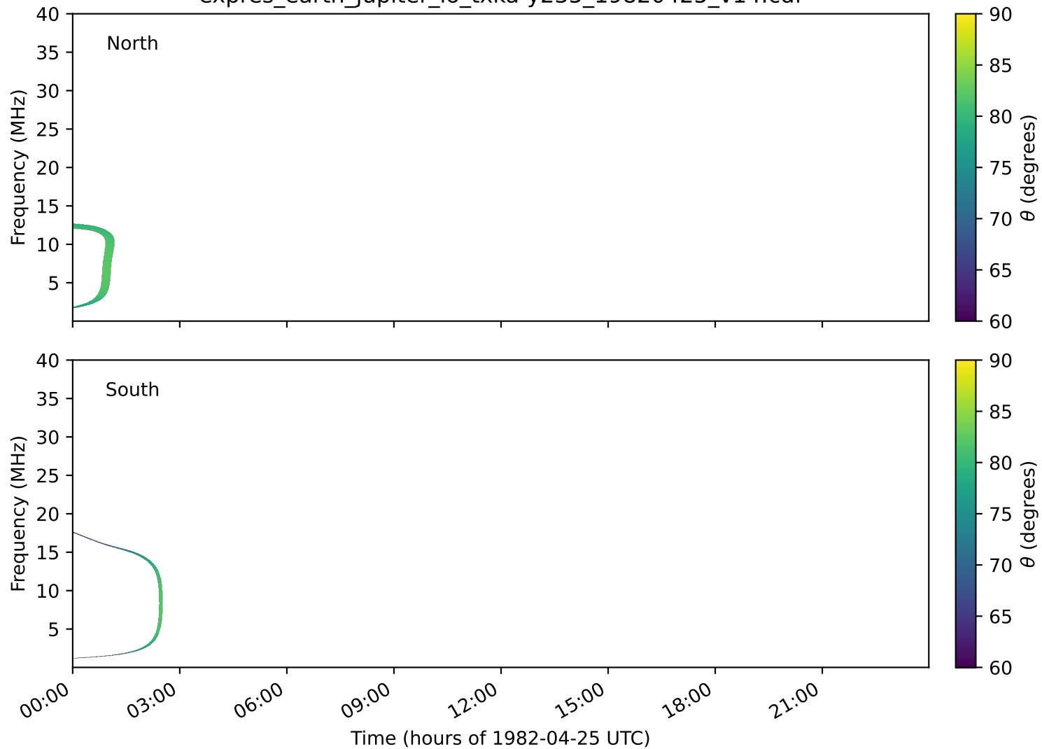
expres_earth_jupiter_io_txka-y235_19820425_v14.cdf
