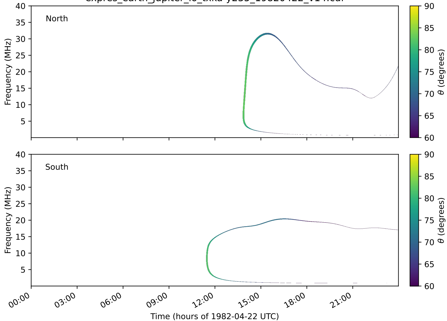
expres_earth_jupiter_io_txka-y235_19820422_v14.cdf
