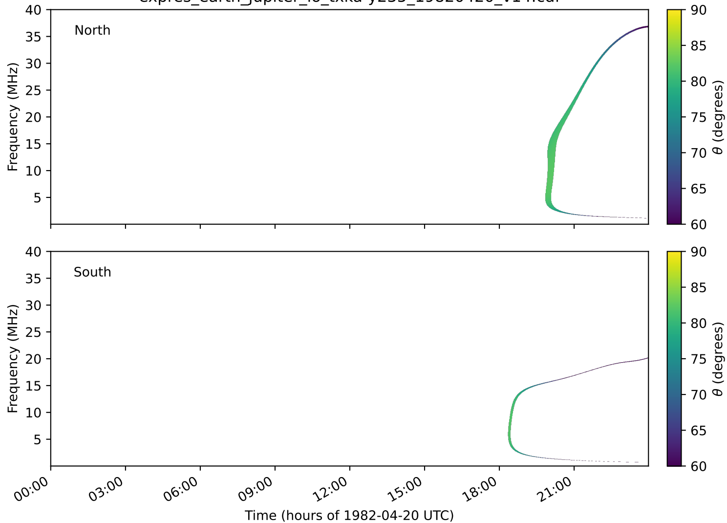
expres_earth_jupiter_io_txka-y235_19820420_v14.cdf
