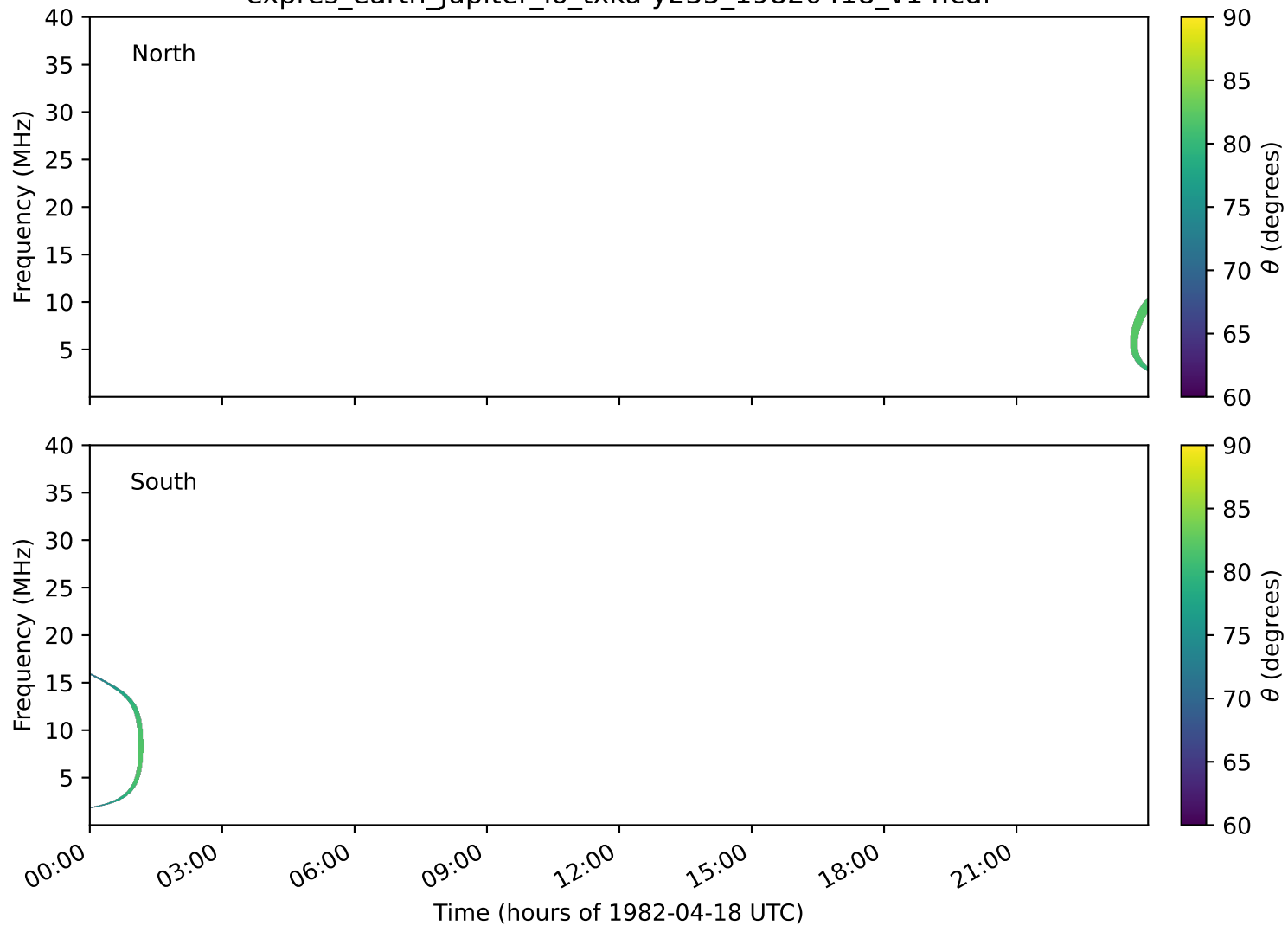
expres_earth_jupiter_io_txka-y235_19820418_v14.cdf
