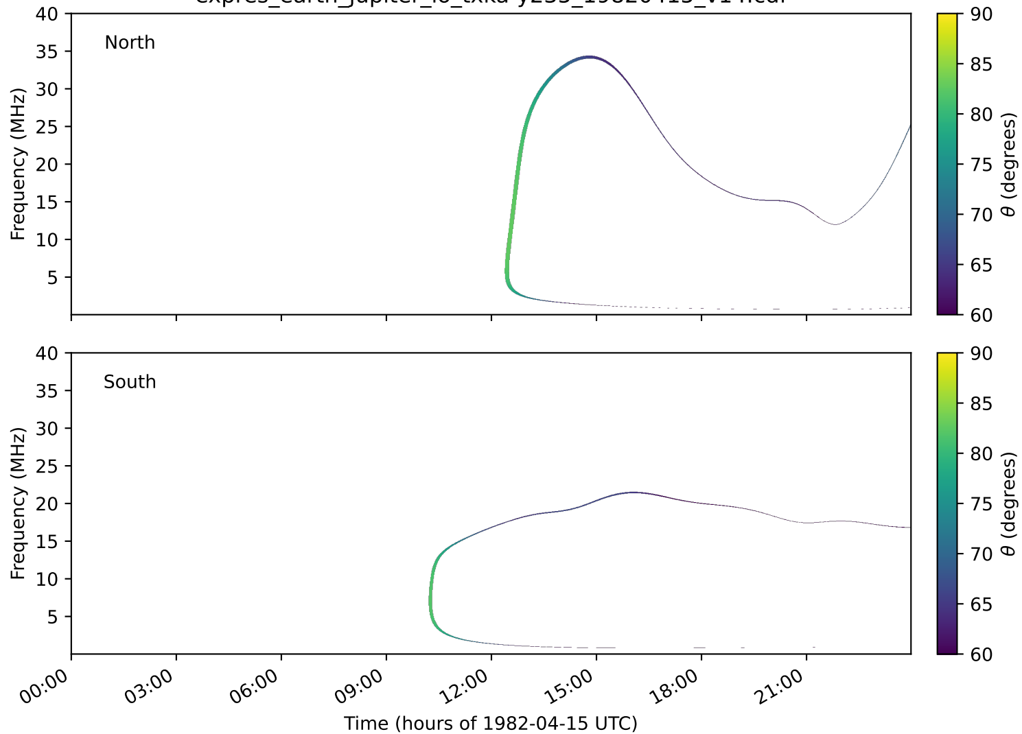
expres_earth_jupiter_io_txka-y235_19820415_v14.cdf
