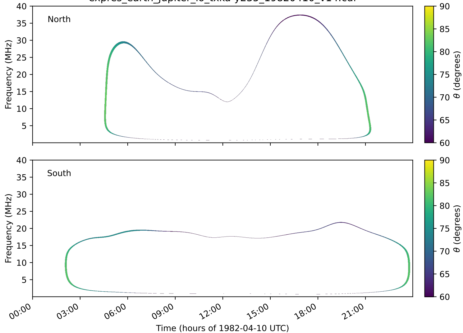
expres_earth_jupiter_io_txka-y235_19820410_v14.cdf
