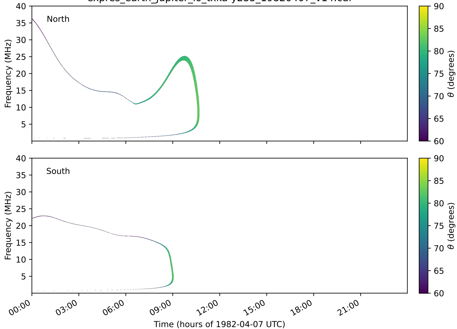
expres_earth_jupiter_io_txka-y235_19820407_v14.cdf
