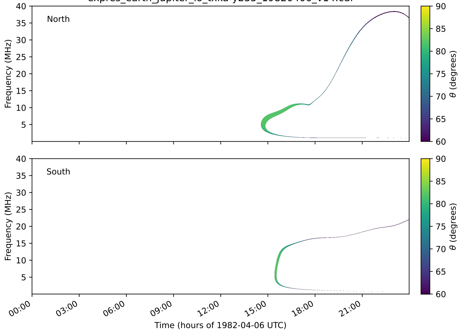
expres_earth_jupiter_io_txka-y235_19820406_v14.cdf
