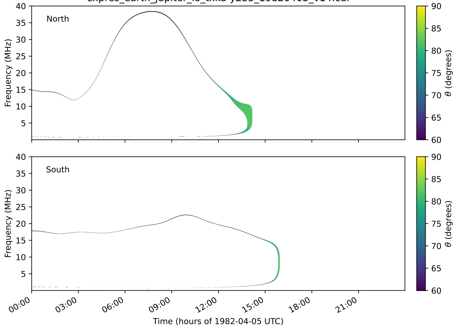
expres_earth_jupiter_io_txka-y235_19820405_v14.cdf
