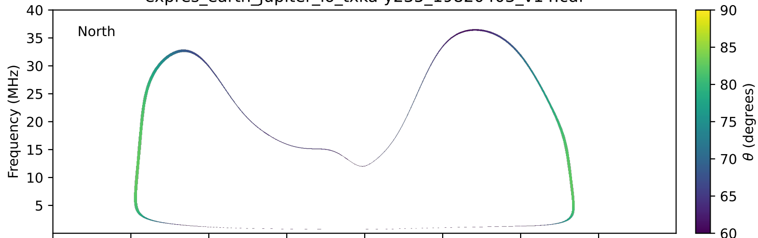
expres_earth_jupiter_io_txka-y235_19820403_v14.cdf
