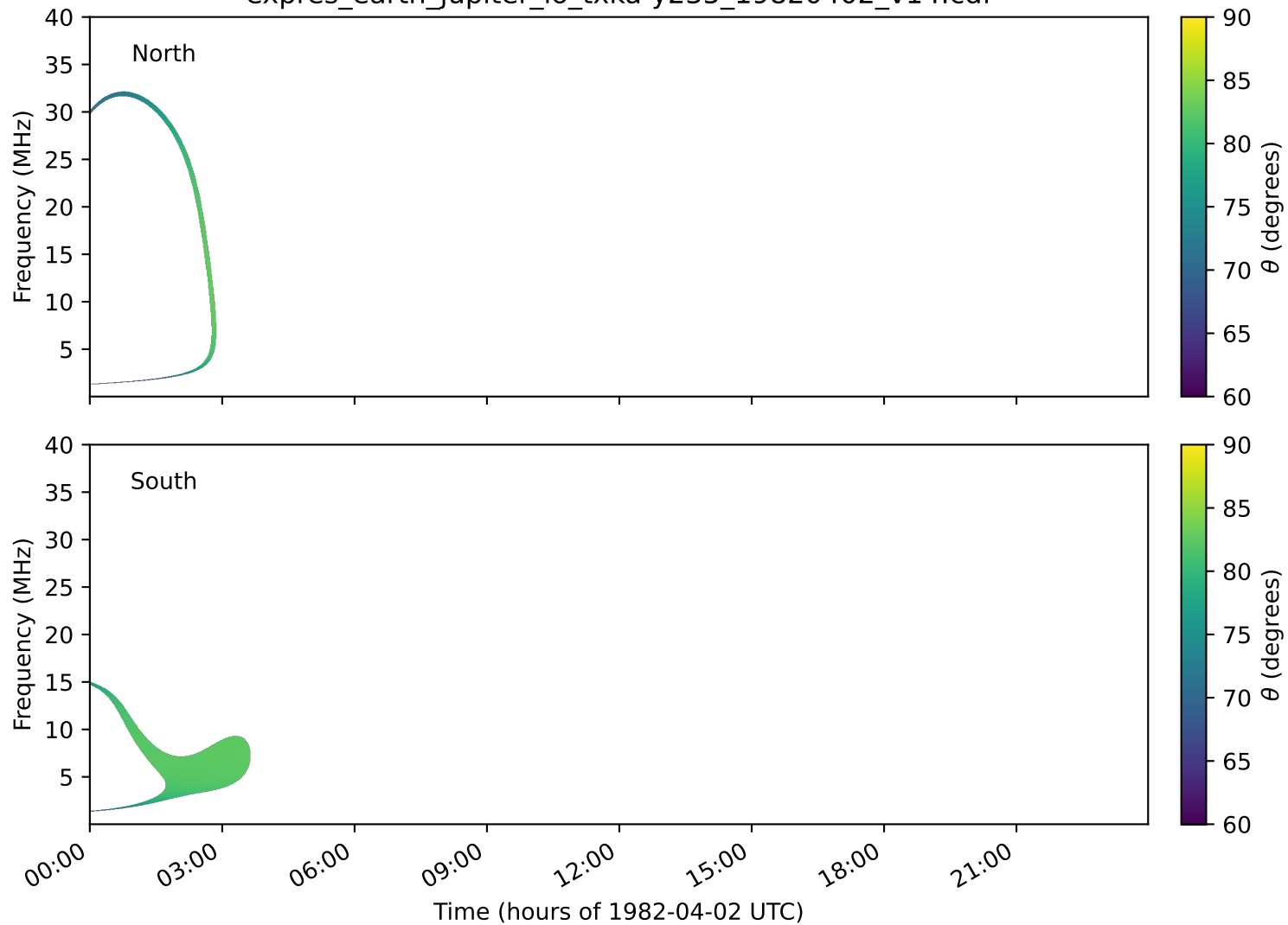
expres_earth_jupiter_io_txka-y235_19820402_v14.cdf
