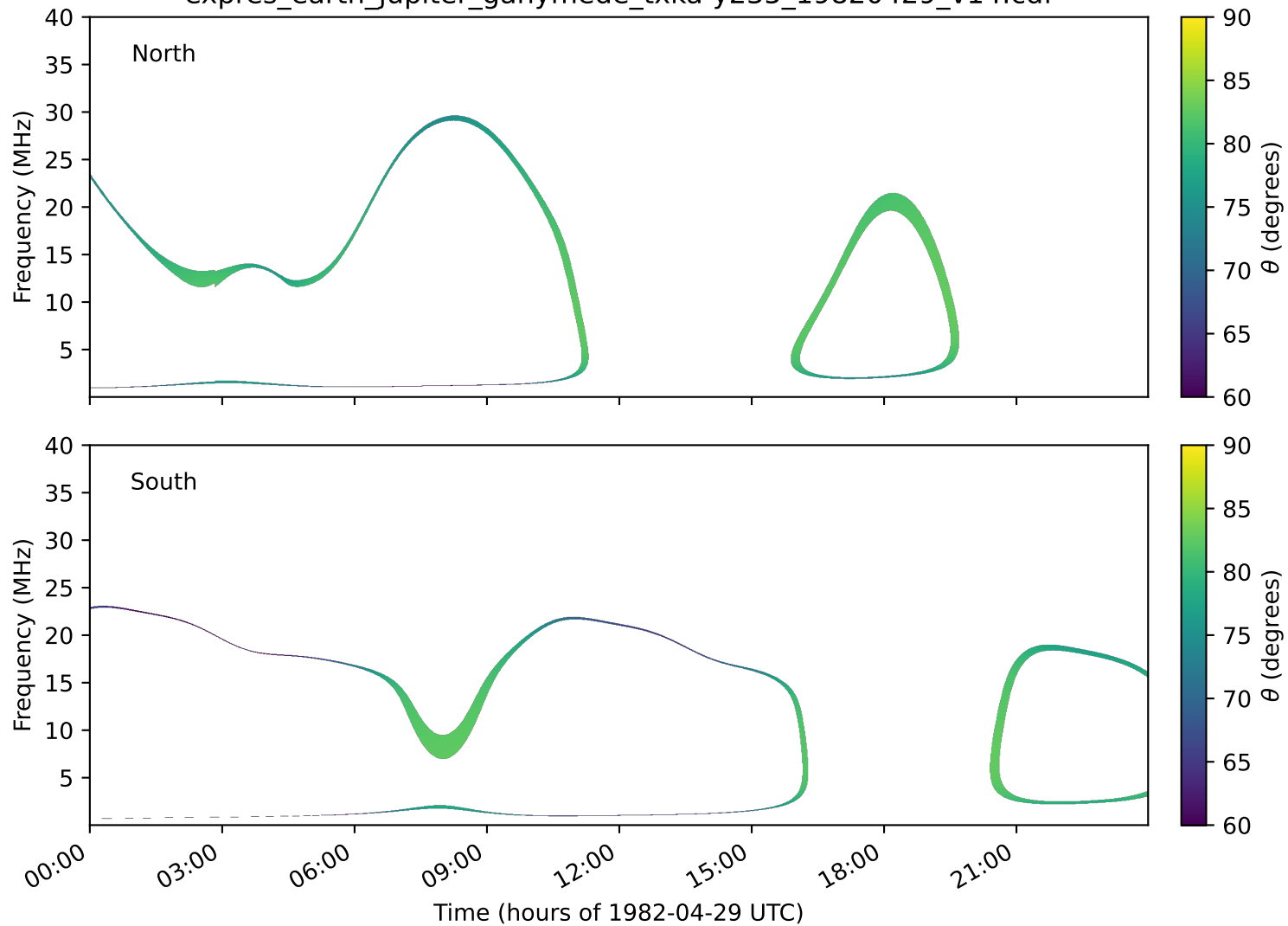
expres_earth_jupiter_ganymede_txka-y235_19820429_v14.cdf
