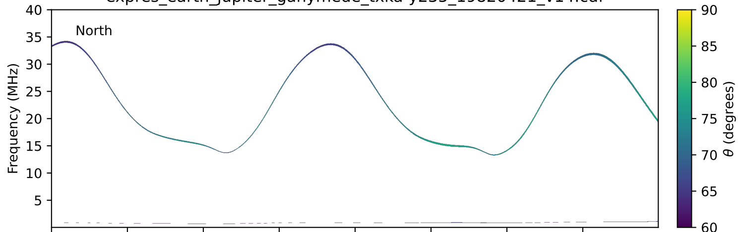
expres_earth_jupiter_ganymede_txka-y235_19820421_v14.cdf
