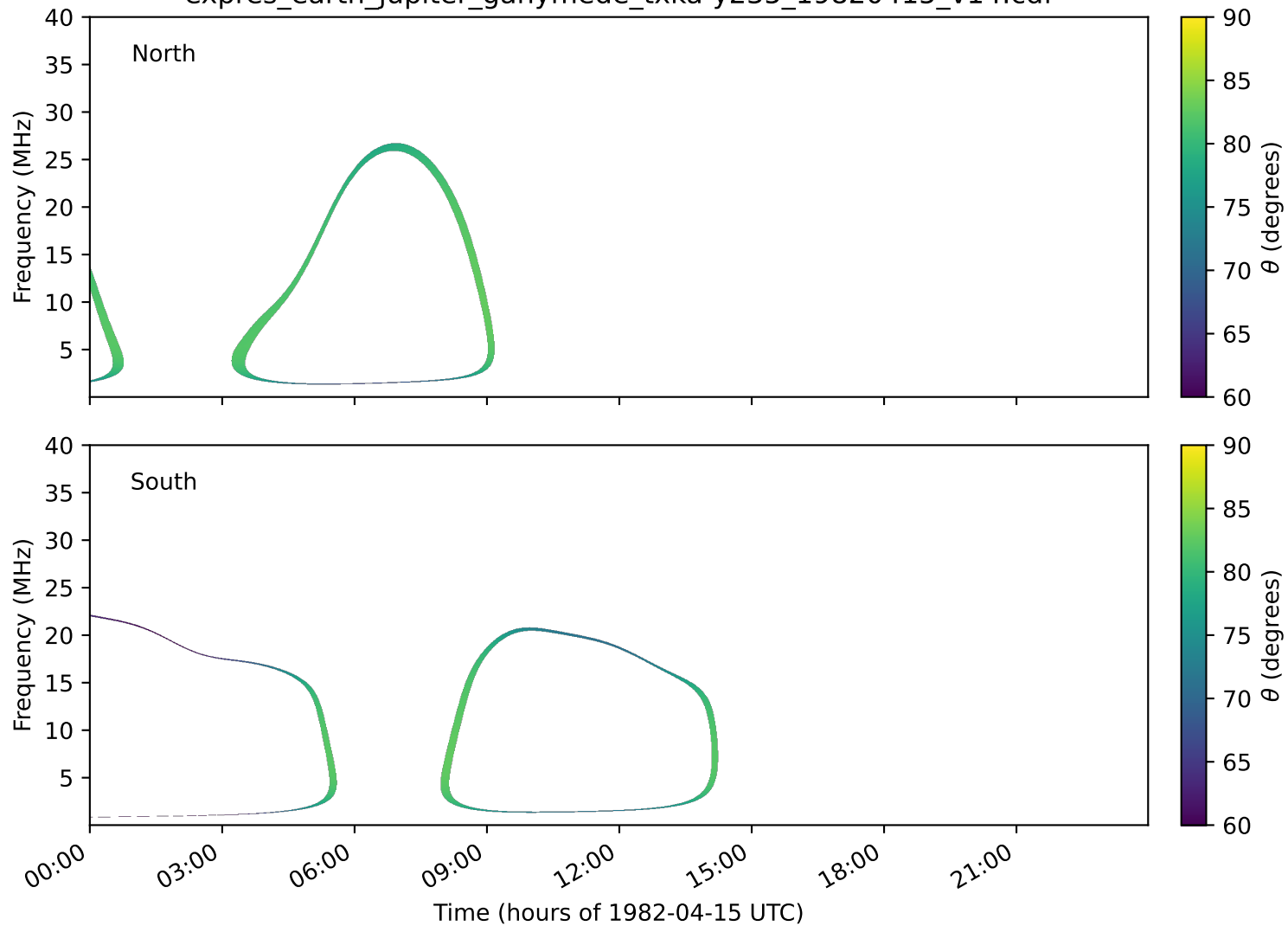
expres_earth_jupiter_ganymede_txka-y235_19820415_v14.cdf
