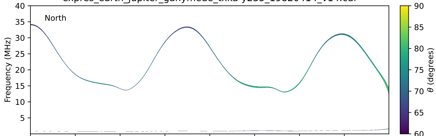
expres_earth_jupiter_ganymede_txka-y235_19820414_v14.cdf
