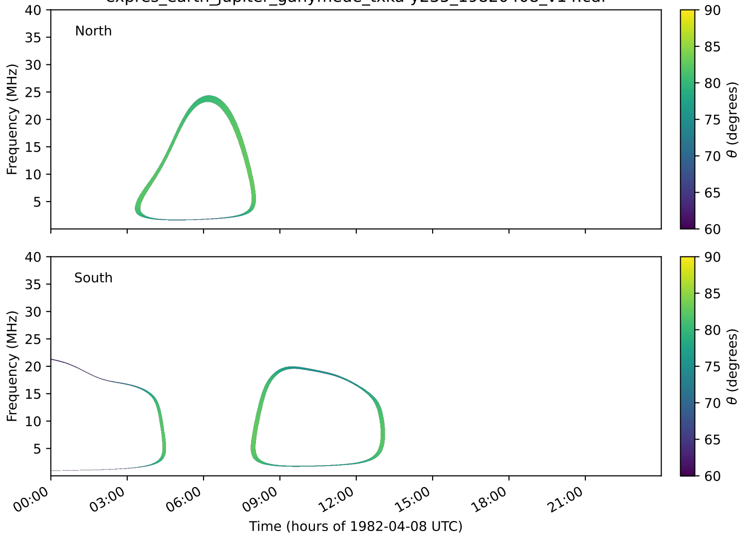
expres_earth_jupiter_ganymede_txka-y235_19820408_v14.cdf
