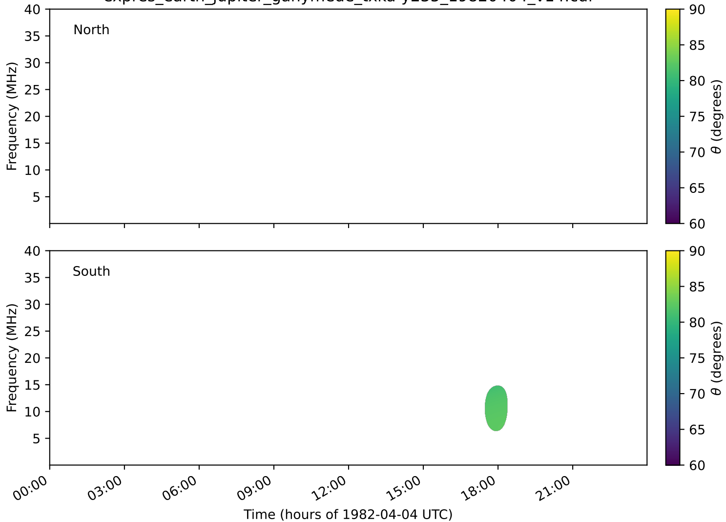
expres_earth_jupiter_ganymede_txka-y235_19820404_v14.cdf
