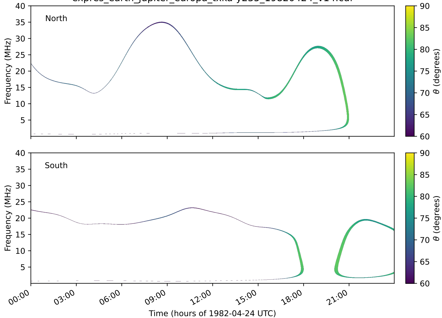
expres_earth_jupiter_europa_txka-y235_19820424_v14.cdf
