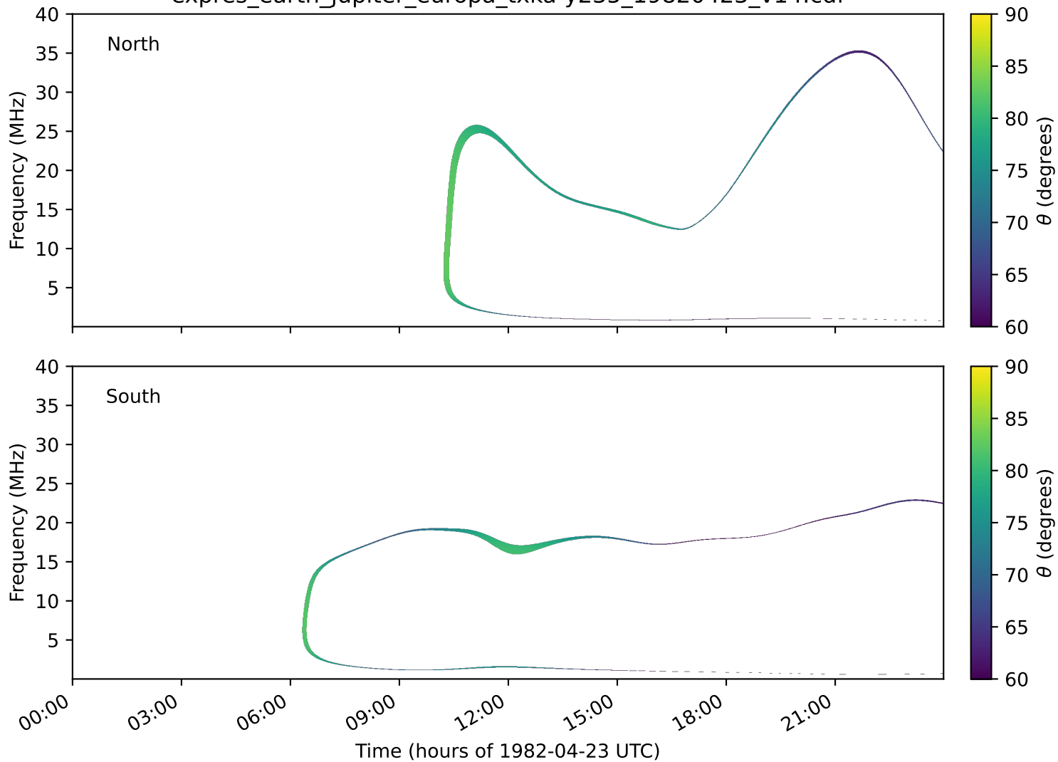
expres_earth_jupiter_europa_txka-y235_19820423_v14.cdf
