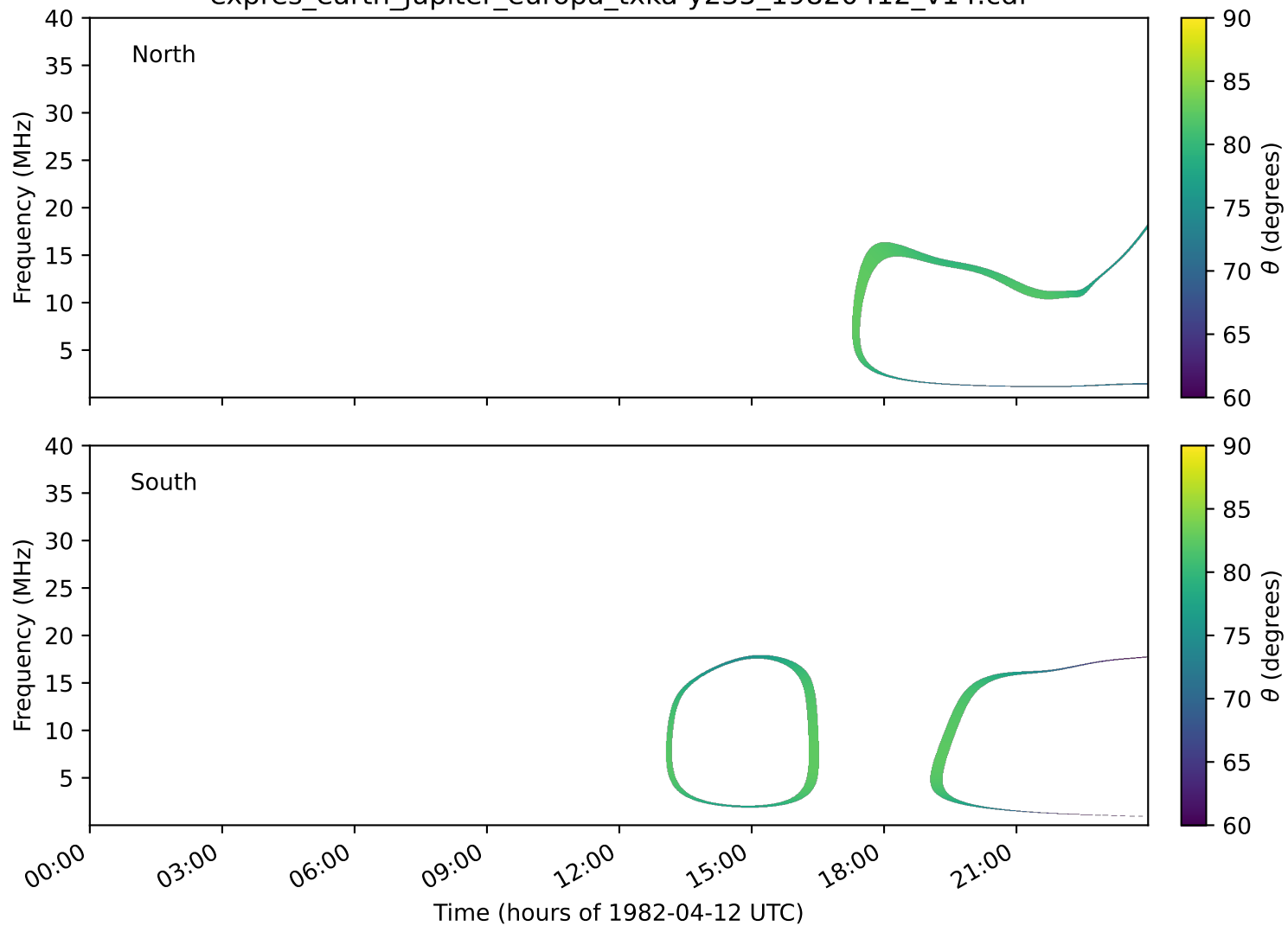
expres_earth_jupiter_europa_txka-y235_19820412_v14.cdf
