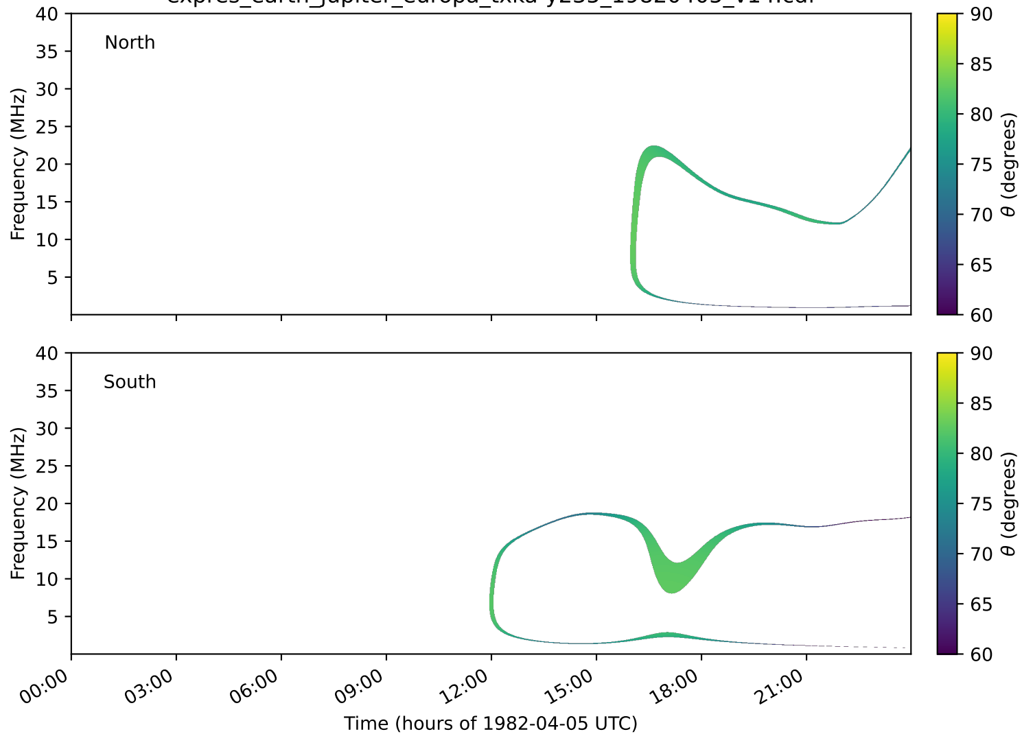
expres_earth_jupiter_europa_txka-y235_19820405_v14.cdf
