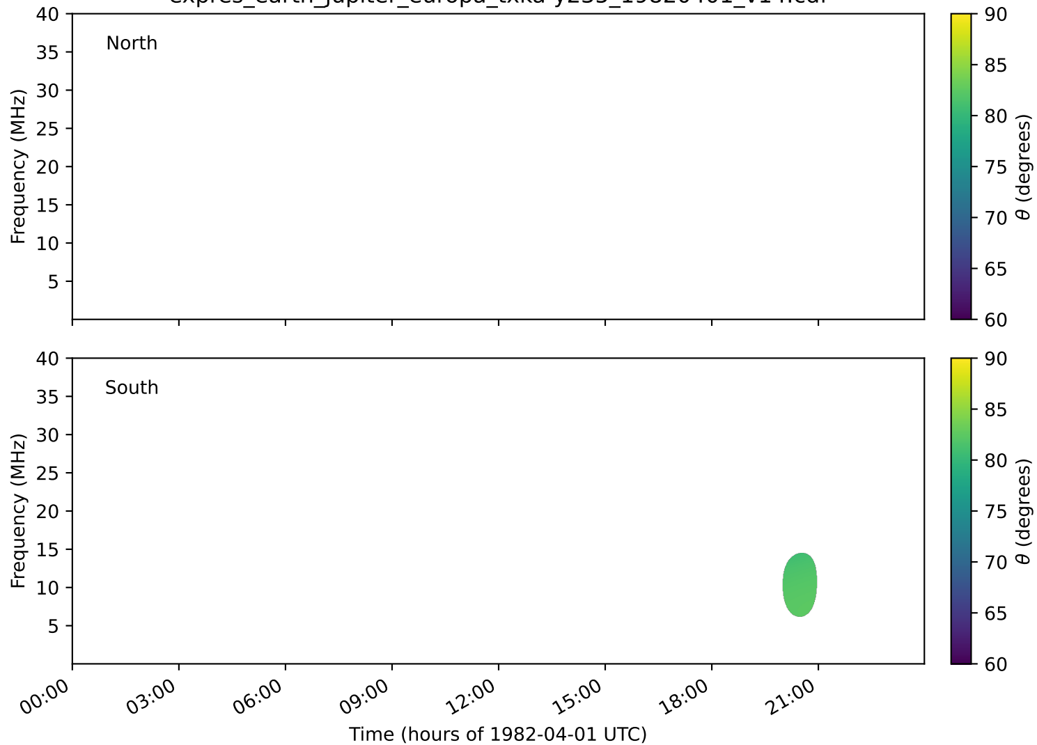
expres_earth_jupiter_europa_txka-y235_19820401_v14.cdf
