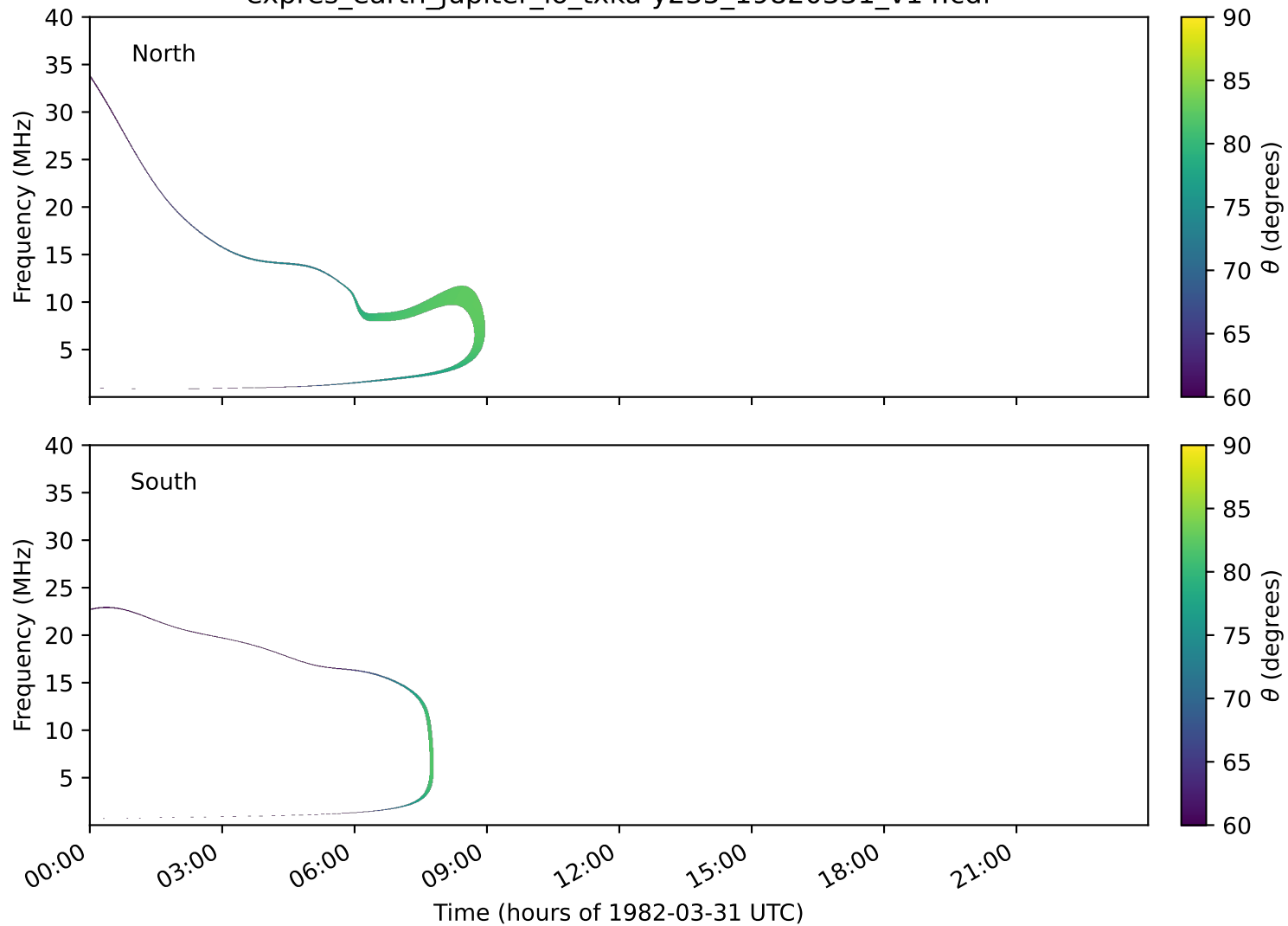
expres_earth_jupiter_io_txka-y235_19820331_v14.cdf
