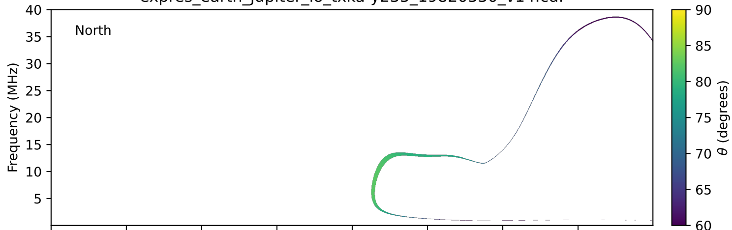
expres_earth_jupiter_io_txka-y235_19820330_v14.cdf
