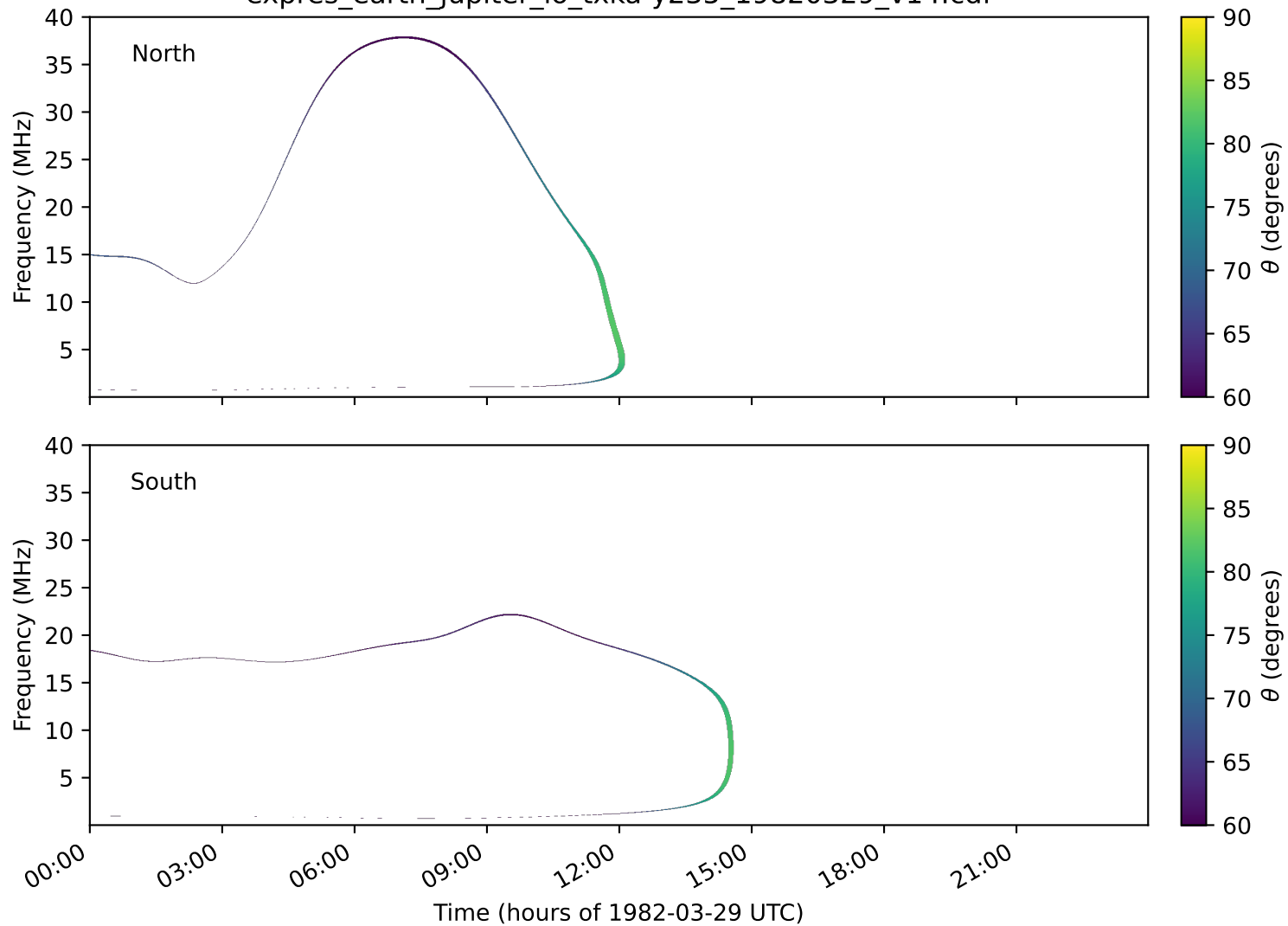
expres_earth_jupiter_io_txka-y235_19820329_v14.cdf
