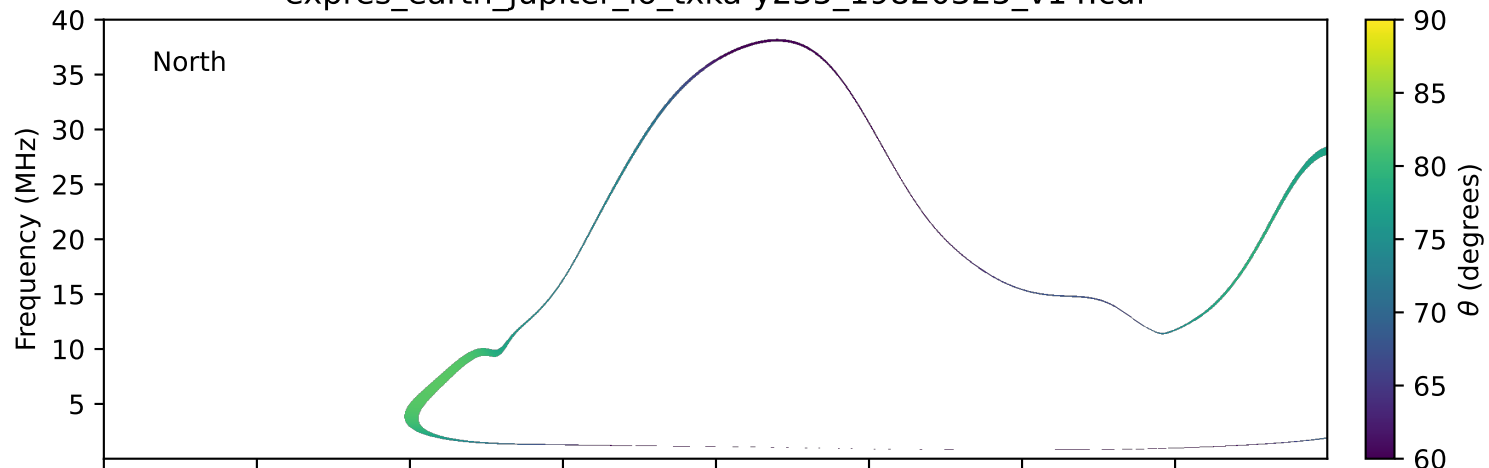
expres_earth_jupiter_io_txka-y235_19820325_v14.cdf
