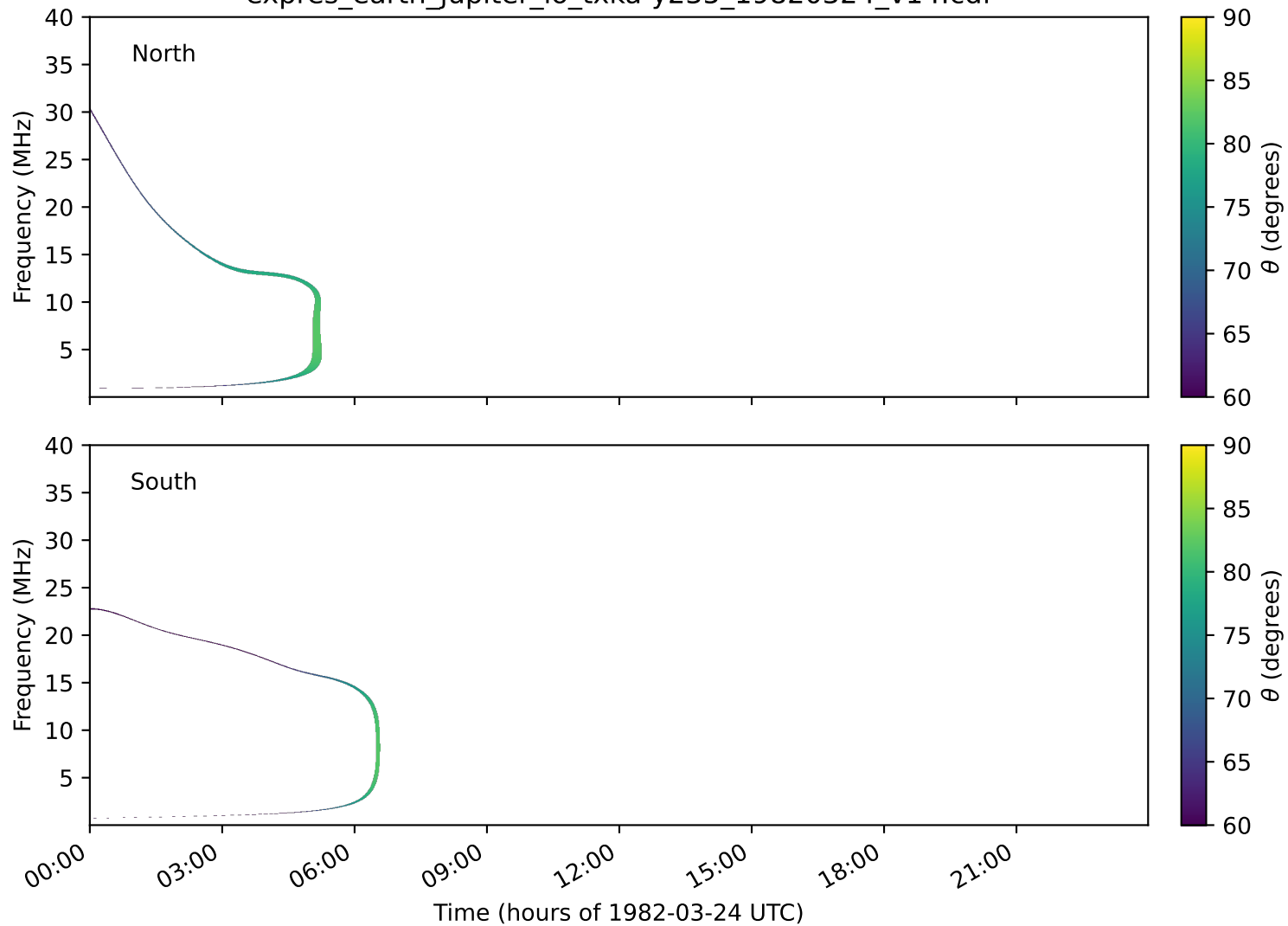
expres_earth_jupiter_io_txka-y235_19820324_v14.cdf
