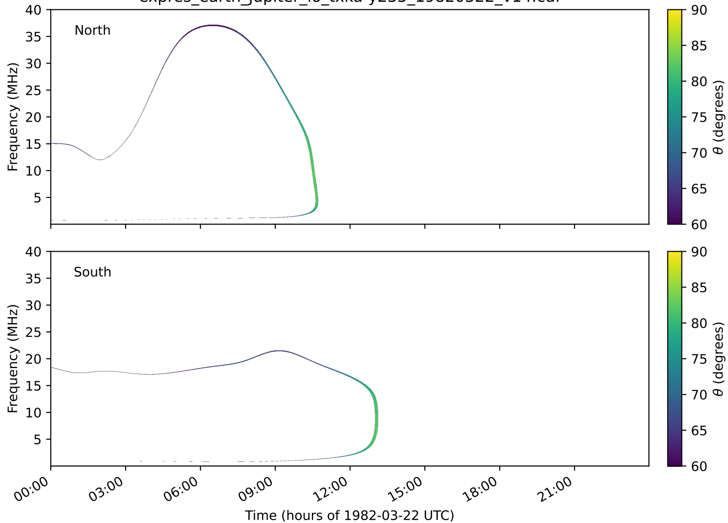
expres_earth_jupiter_io_txka-y235_19820322_v14.cdf
