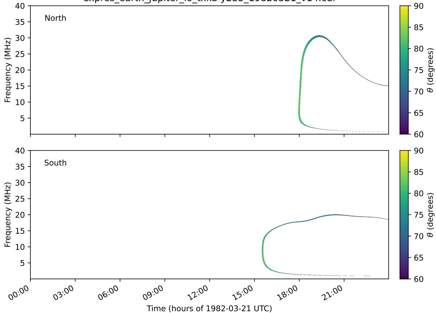
expres_earth_jupiter_io_txka-y235_19820321_v14.cdf
