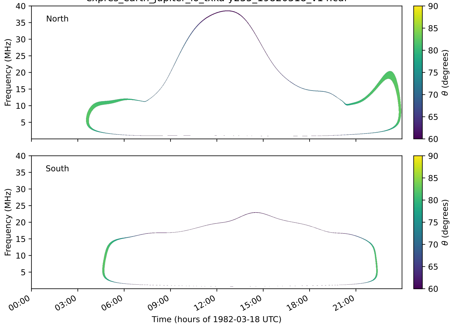
expres_earth_jupiter_io_txka-y235_19820318_v14.cdf
