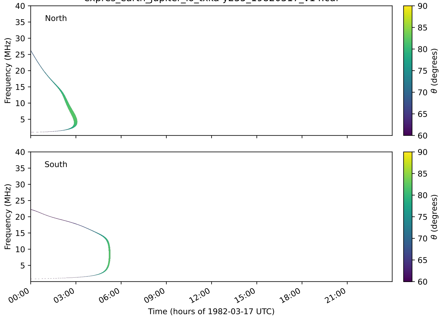
expres_earth_jupiter_io_txka-y235_19820317_v14.cdf
