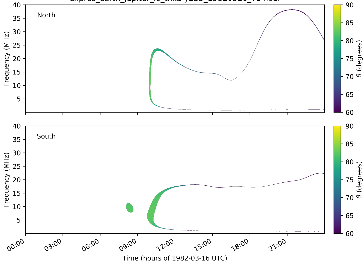
expres_earth_jupiter_io_txka-y235_19820316_v14.cdf
