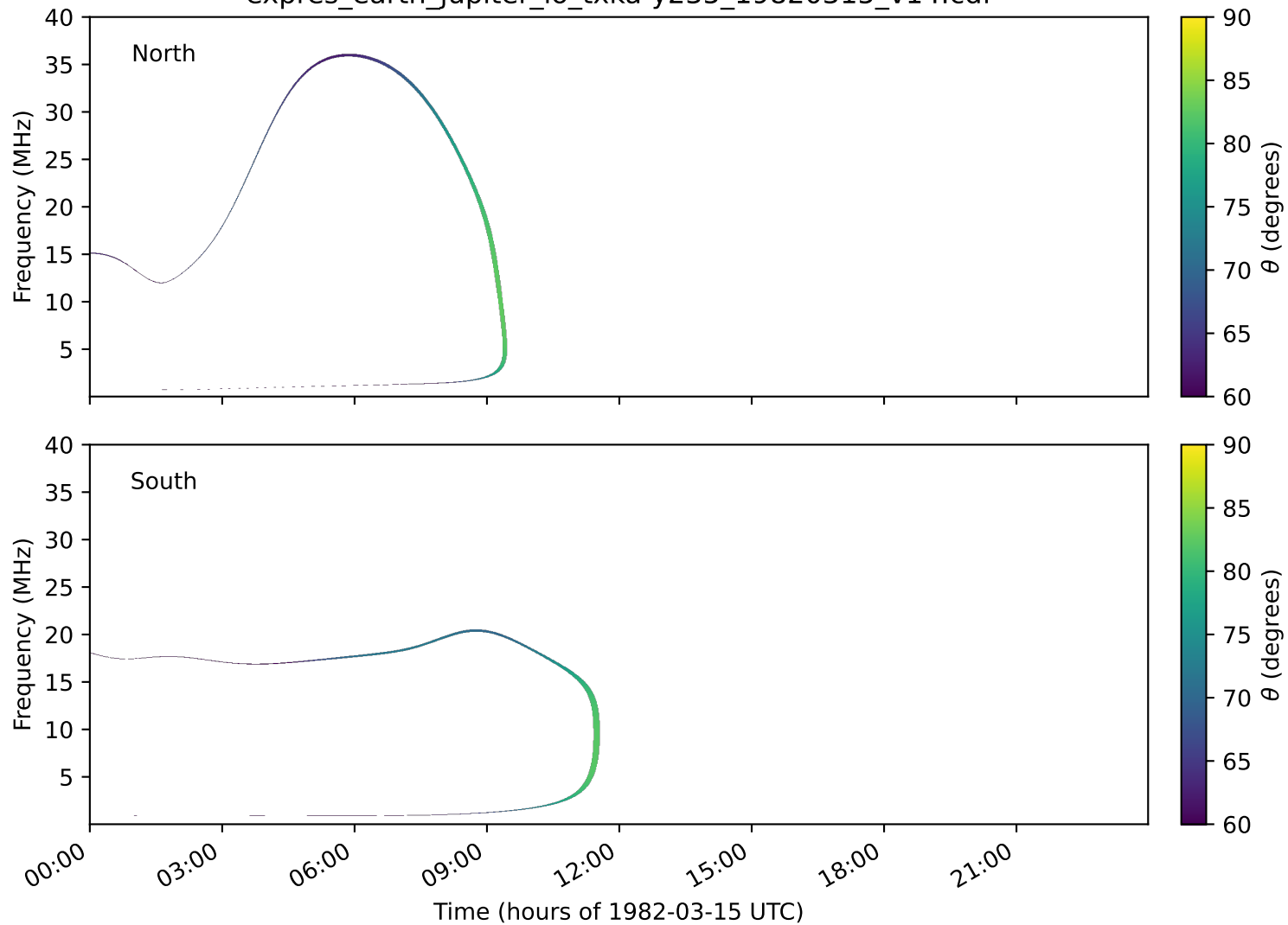
expres_earth_jupiter_io_txka-y235_19820315_v14.cdf
