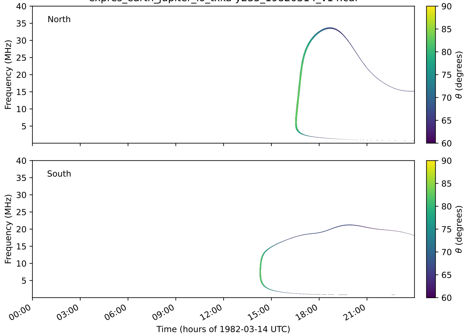
expres_earth_jupiter_io_txka-y235_19820314_v14.cdf
