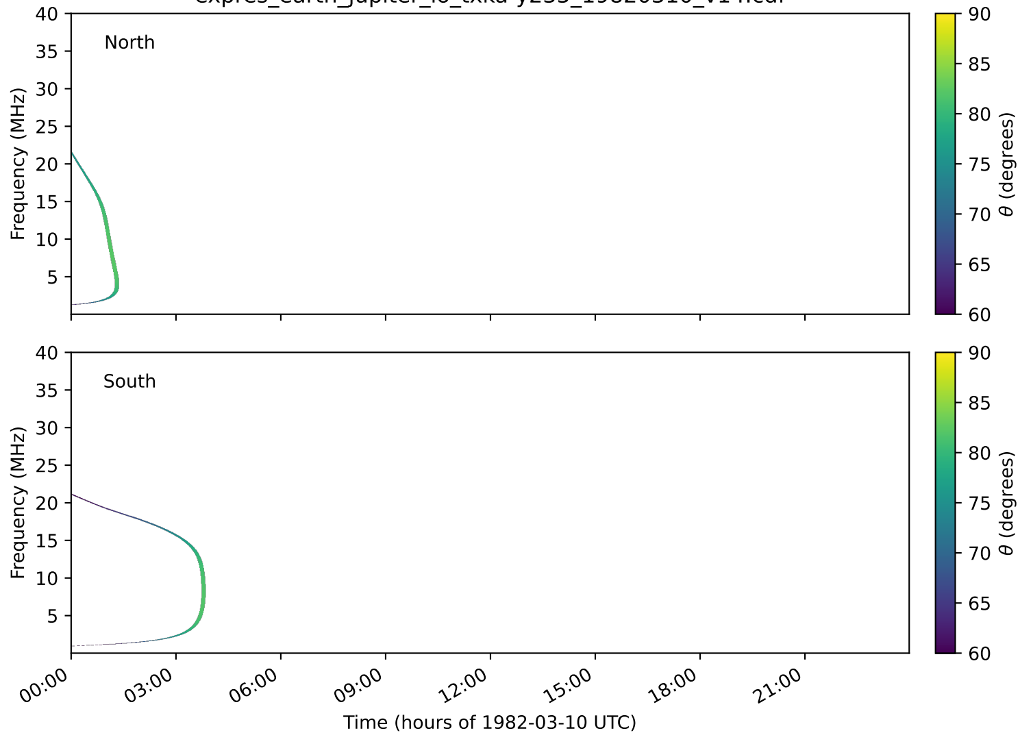
expres_earth_jupiter_io_txka-y235_19820310_v14.cdf
