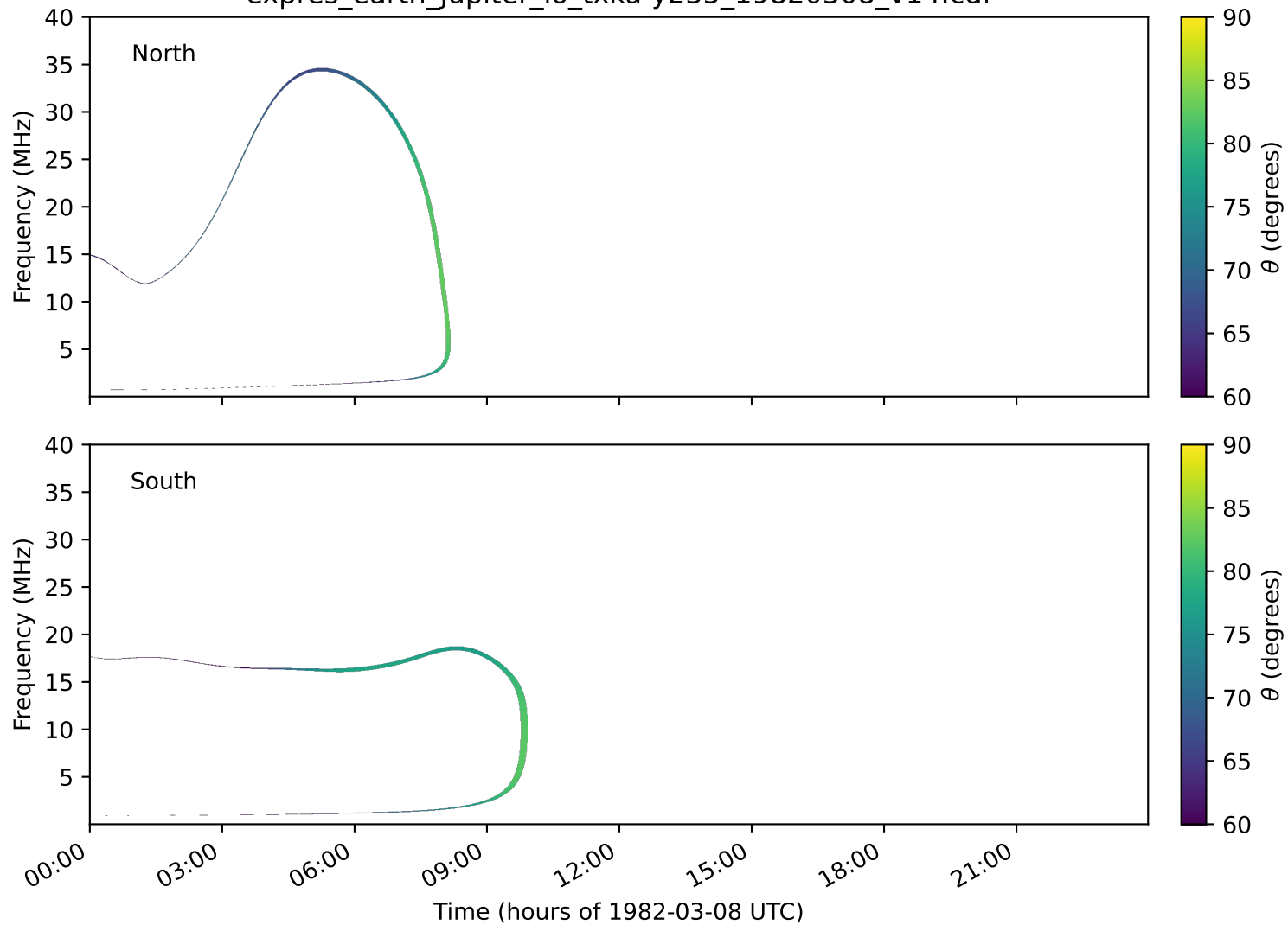
expres_earth_jupiter_io_txka-y235_19820308_v14.cdf
