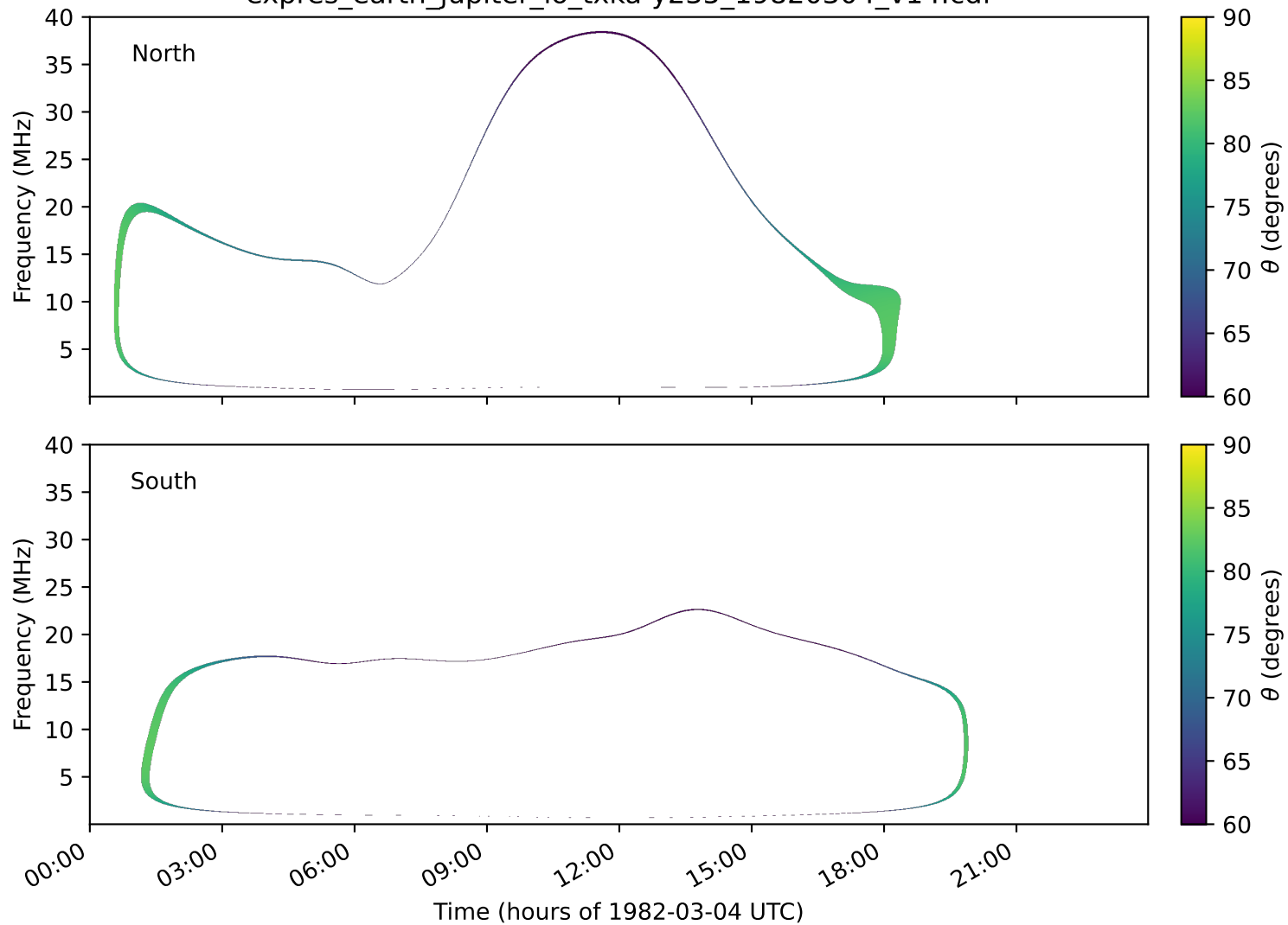
expres_earth_jupiter_io_txka-y235_19820304_v14.cdf
