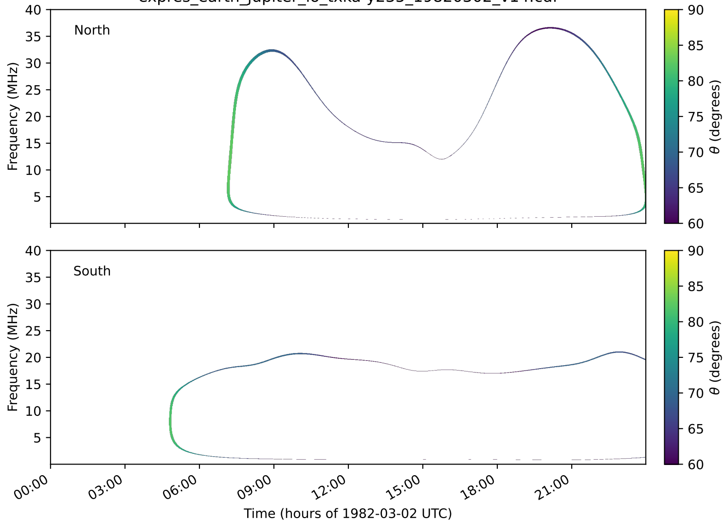
expres_earth_jupiter_io_txka-y235_19820302_v14.cdf
