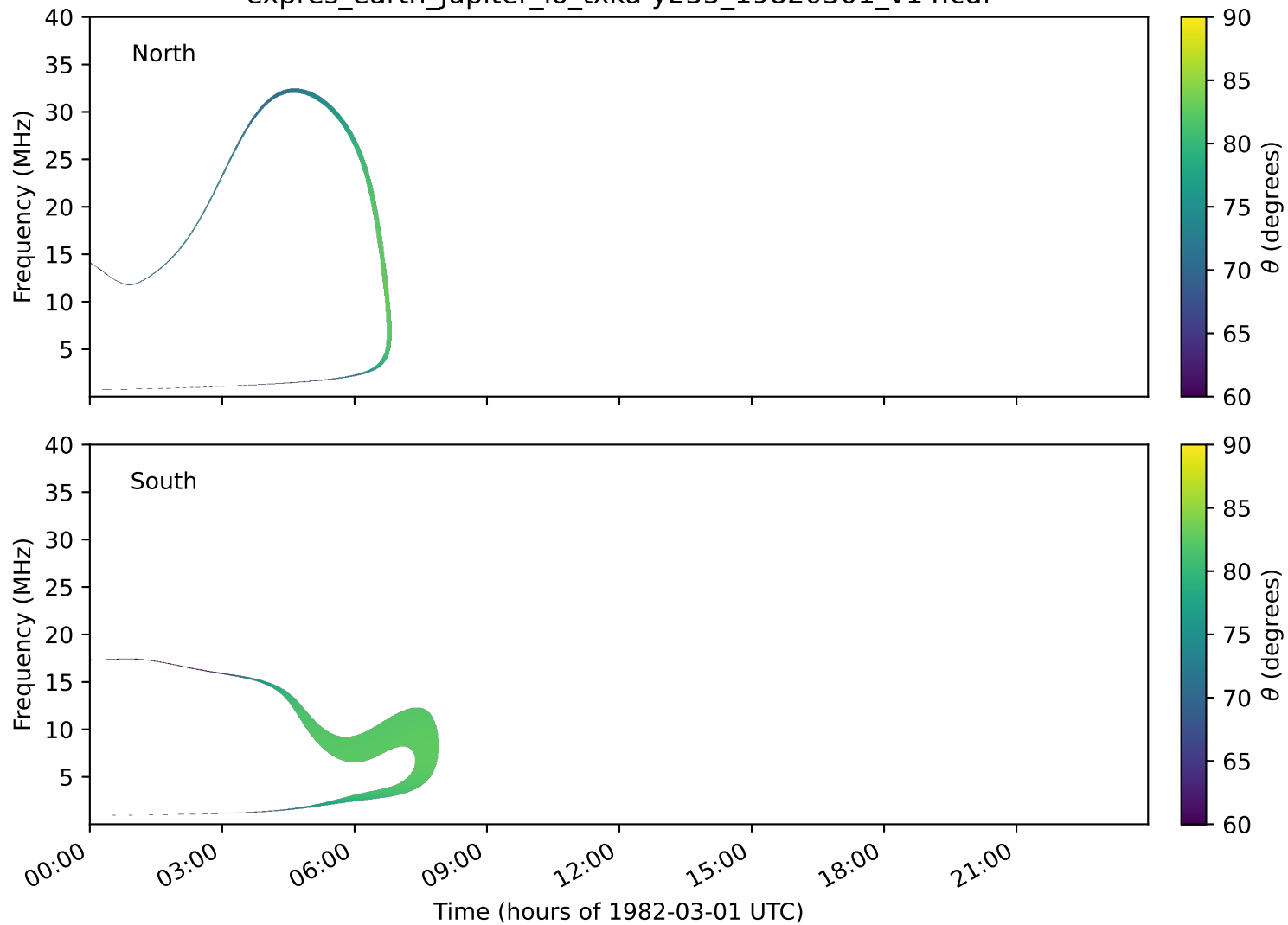
expres_earth_jupiter_io_txka-y235_19820301_v14.cdf
